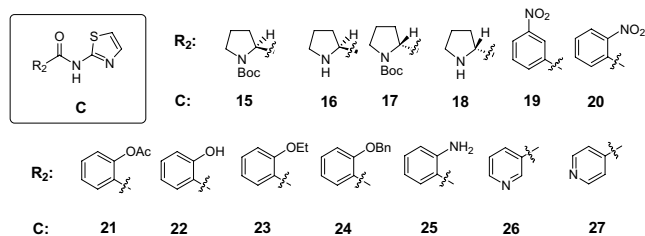
Figure 2. Compounds 15–27.
