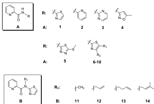
Figure 1. Compounds 1–14.
